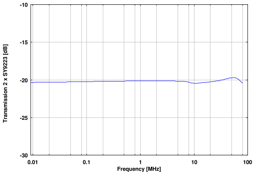
Abb. 1 Transmission zweier SY9223-150 an EuT verbunden Fig. 1: Transmission of two SY9223-150 connected at the EuT port
