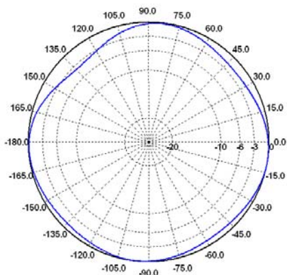
E-Ebene / E-Plane 900 MHz
