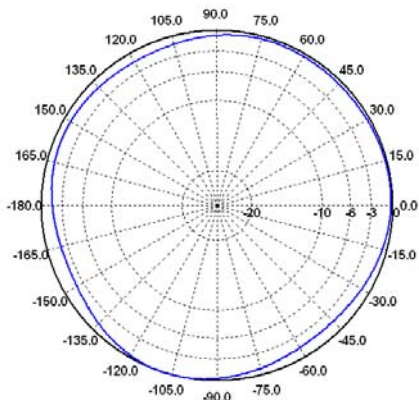
E-Ebene / E-Plane 600 MHz
