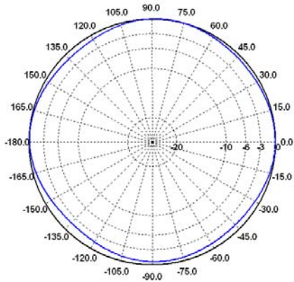
E-Ebene / E-Plane 700 MHz
