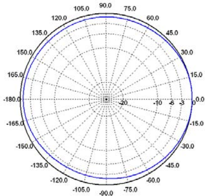
E-Ebene / E-Plane 400 MHz
