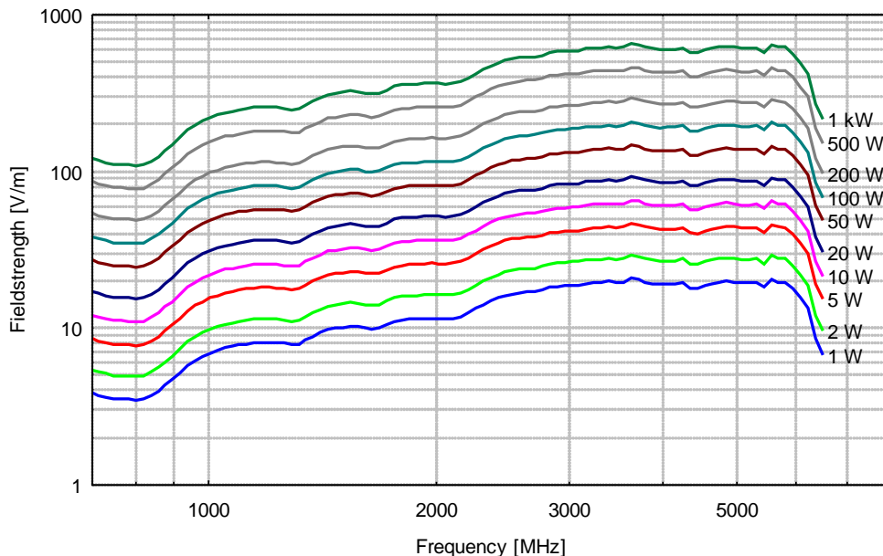
BBHA 9120 J Input Power, Dist. Aperture-EuT: 3 m
