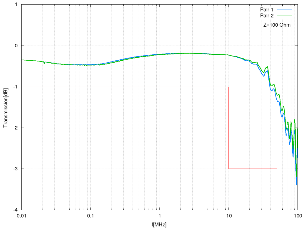
Bild 4: typ. Transmission AE zu EuT (differenziell) Fig. 4: typ. transmission AE – EuT(differential)
