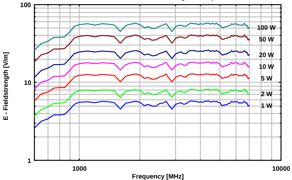
USLP 9142 Generated Fieldstrength 2 m Tip - EuT
