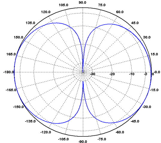
H-Ebene / H-Plane 220 MHz
