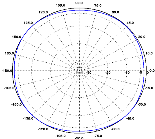
E-Ebene / E-Plane 230 MHz
