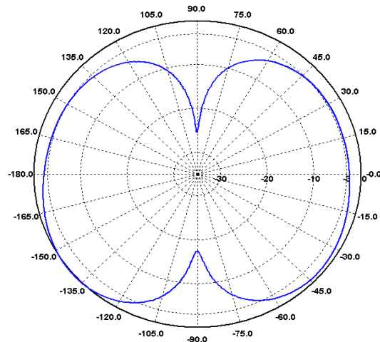
H-Ebene / H-Plane 270 MHz
