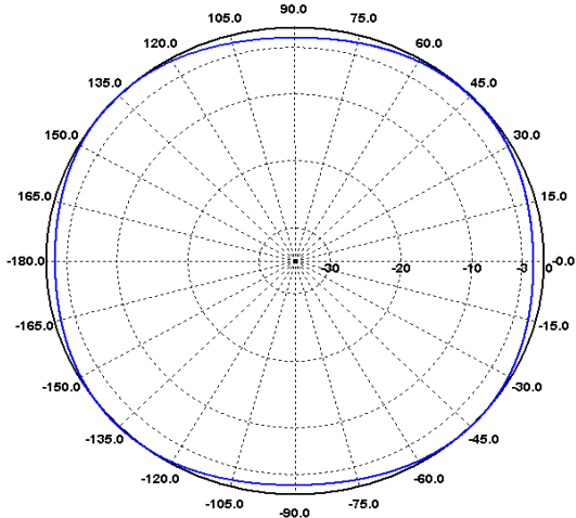
E-Ebene / E-Plane 220 MHz
