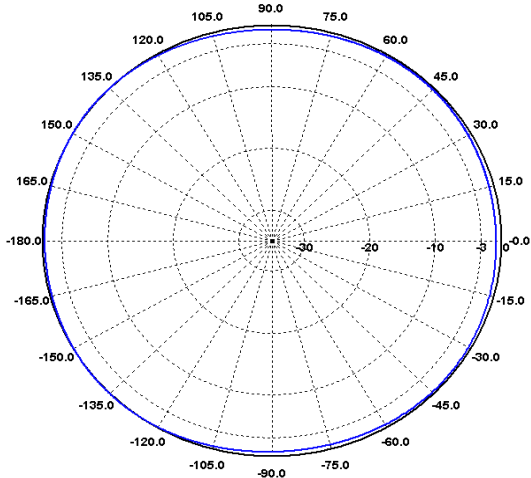
E-Ebene / E-Plane 190 MHz
