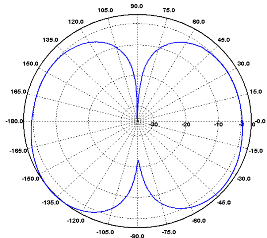
H-Ebene / H-Plane 300 MHz
