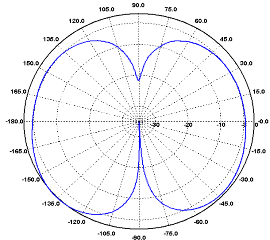
H-Ebene / H-Plane 290 MHz
