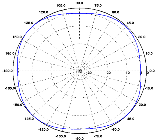
E-Ebene / E-Plane 250 MHz
