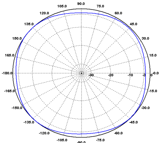
E-Ebene / E-Plane 240 MHz
