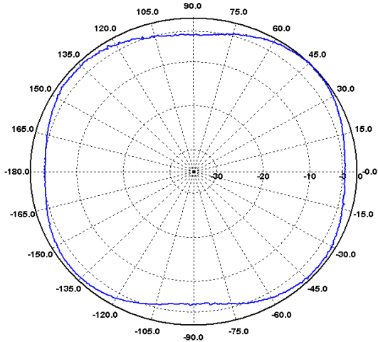
E-Ebene / E-Plane 280 MHz
