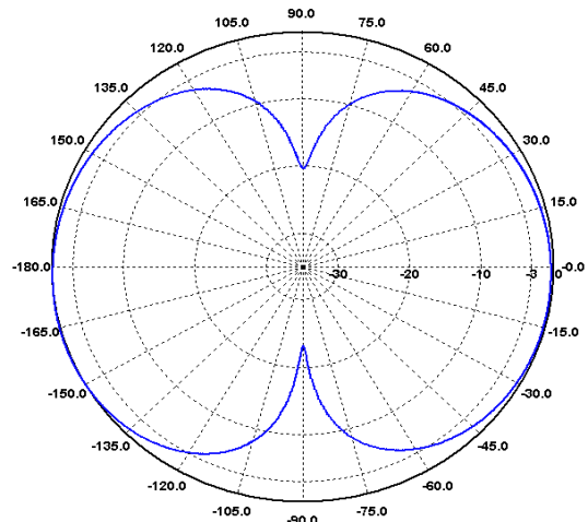
H-Ebene / H-Plane 210 MHz
