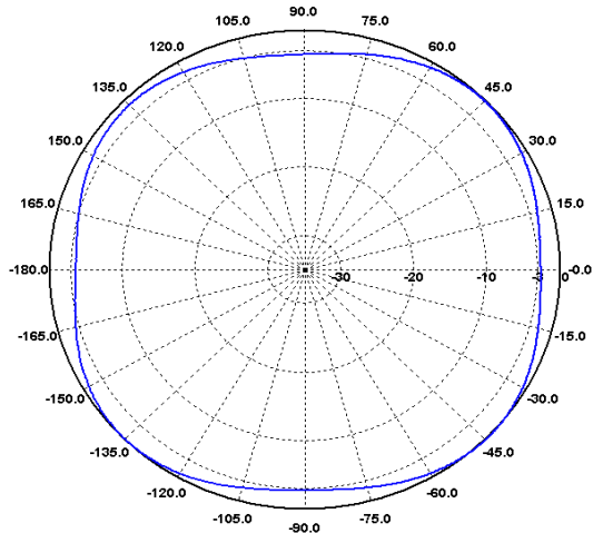
E-Ebene / E-Plane 260 MHz
