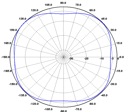
E-Ebene / E-Plane 300 MHz
