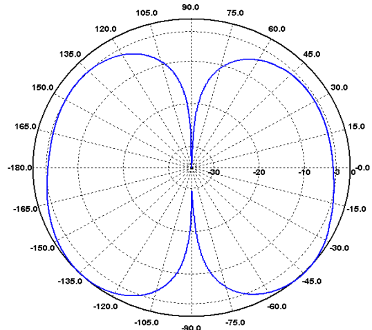
H-Ebene / H-Plane 320 MHz
