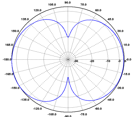
H-Ebene / H-Plane 200 MHz
