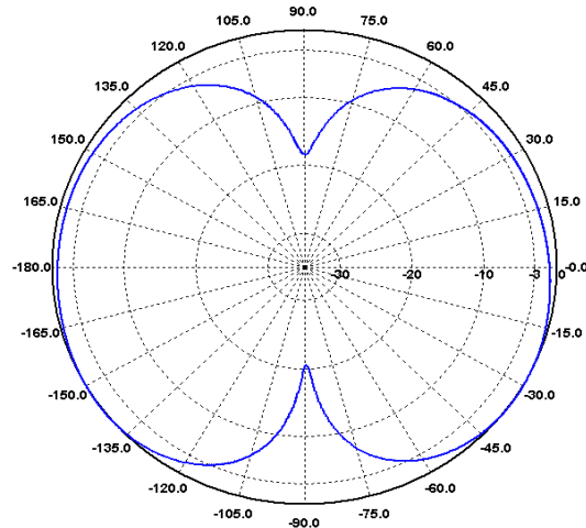
H-Ebene / H-Plane 250 MHz
