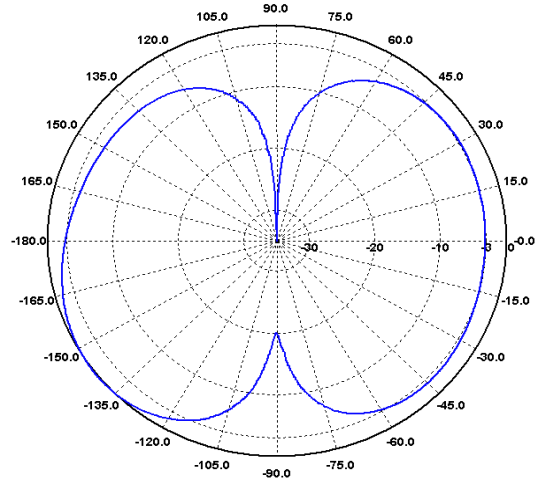
H-Ebene / H-Plane 280 MHz
