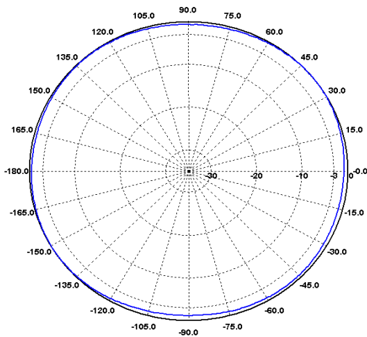
E-Ebene / E-Plane 170 MHz
