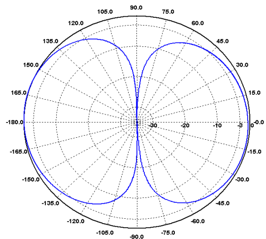
H-Ebene / H-Plane 180 MHz
