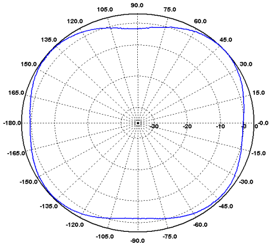
E-Ebene / E-Plane 290 MHz
