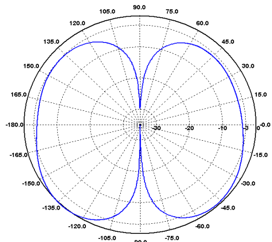
H-Ebene / H-Plane 330 MHz
