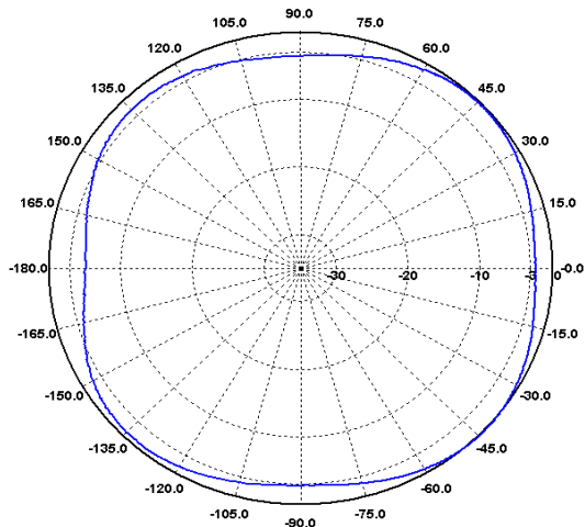
E-Ebene / E-Plane 270 MHz
