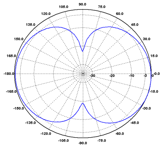
H-Ebene / H-Plane 170 MHz
