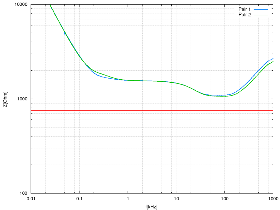
Bild 4: typ. Lastimpedanz (Differenziell) Fig. 4: typ. load impedance (differential)
