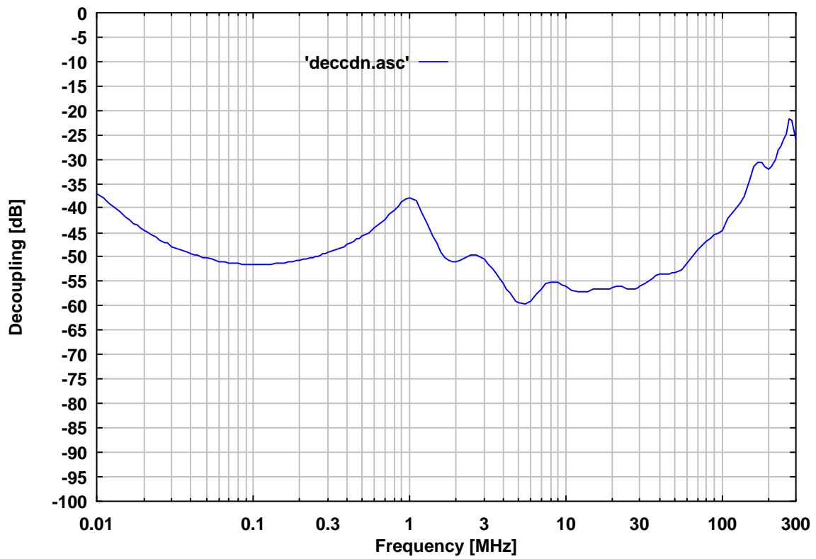
Bild 3: typ. Isolation AE zu HF-Port Fig. 3: typ. isolation AE to RF-port
