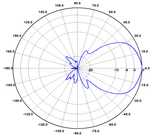
H-Ebene / H-Plane 4 GHz
