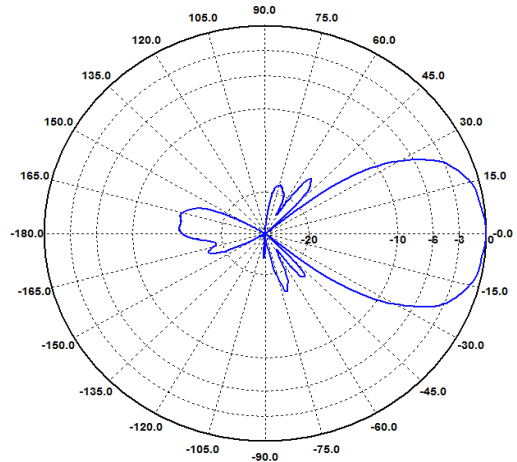
H-Ebene / H-Plane 5 GHz
