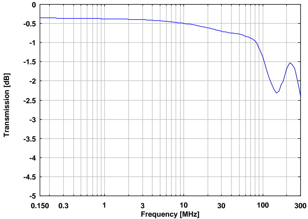
Transmission Differential Mode Signal AE-EuT
