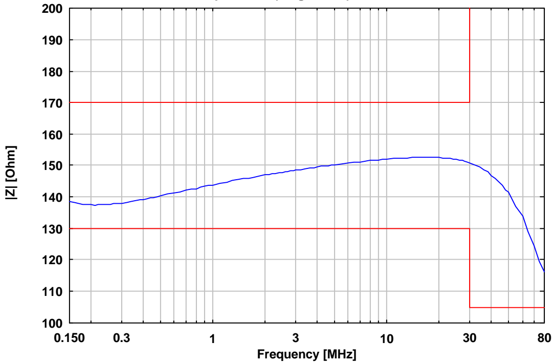
Common Mode Impedance (Magnitude) at EuT-Terminals
